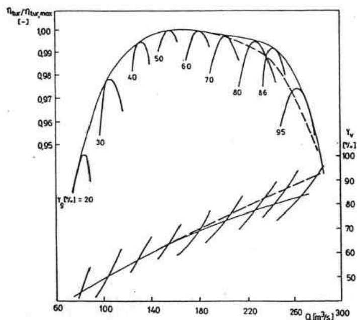
Fig. 9: Existent (dashed line) and optimized "on cam" curve setting at Zlatoličje HPP
