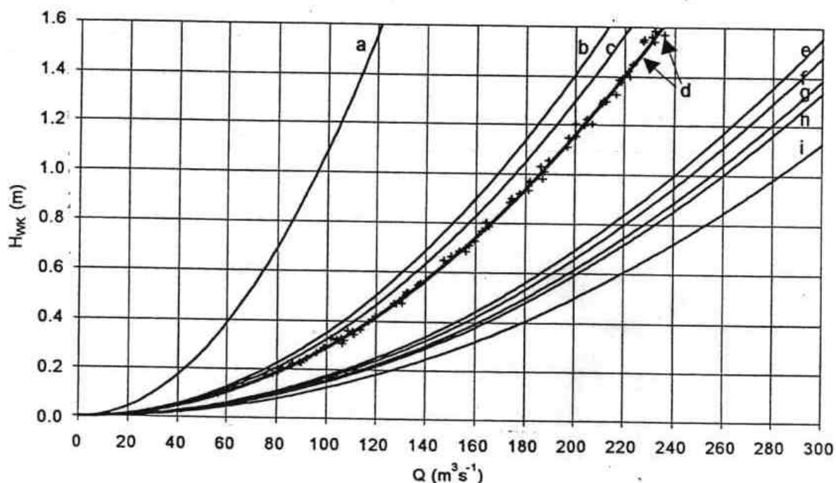
Fig. 1: Influence of different W-K taps on pressure difference: a) Medvode 1(3-4), b) Djale 1, c) Medvode 1 (1-2), d) Zlatoličje 2 (2-3), e) Formin 2 (1-3), f) Zlatoličje 2 (1-2), g) Formin 2 (1-2), h) Fala 10, i) Fala 8
