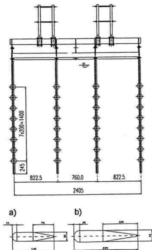
Fig. 5: Current-meter support
