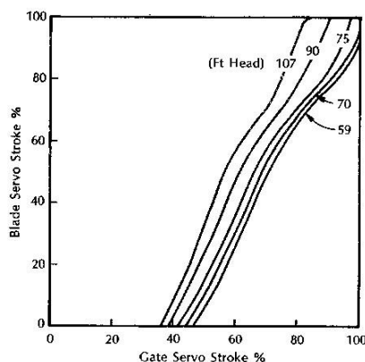
Figure 3. Lines of constant head.
