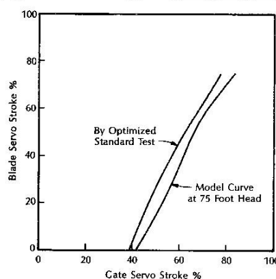
Figure 4. Initial index test results.
